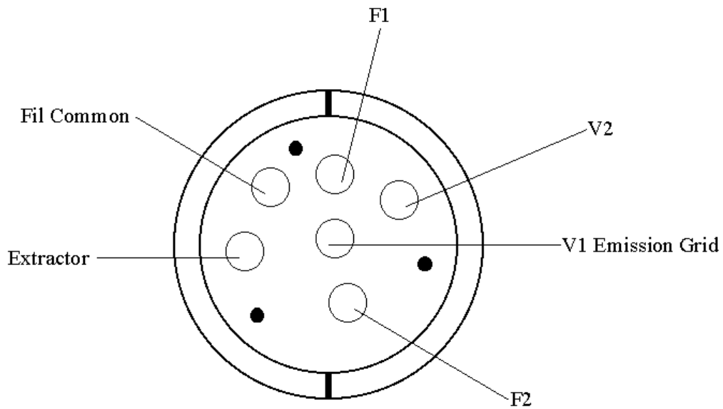
View from top of flange
